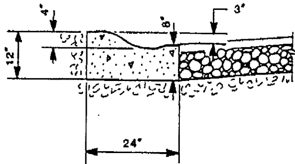
ROLLED CURB NTS
