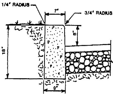
VERTICAL CURB NTS
